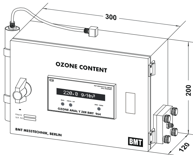
dimensional outline
